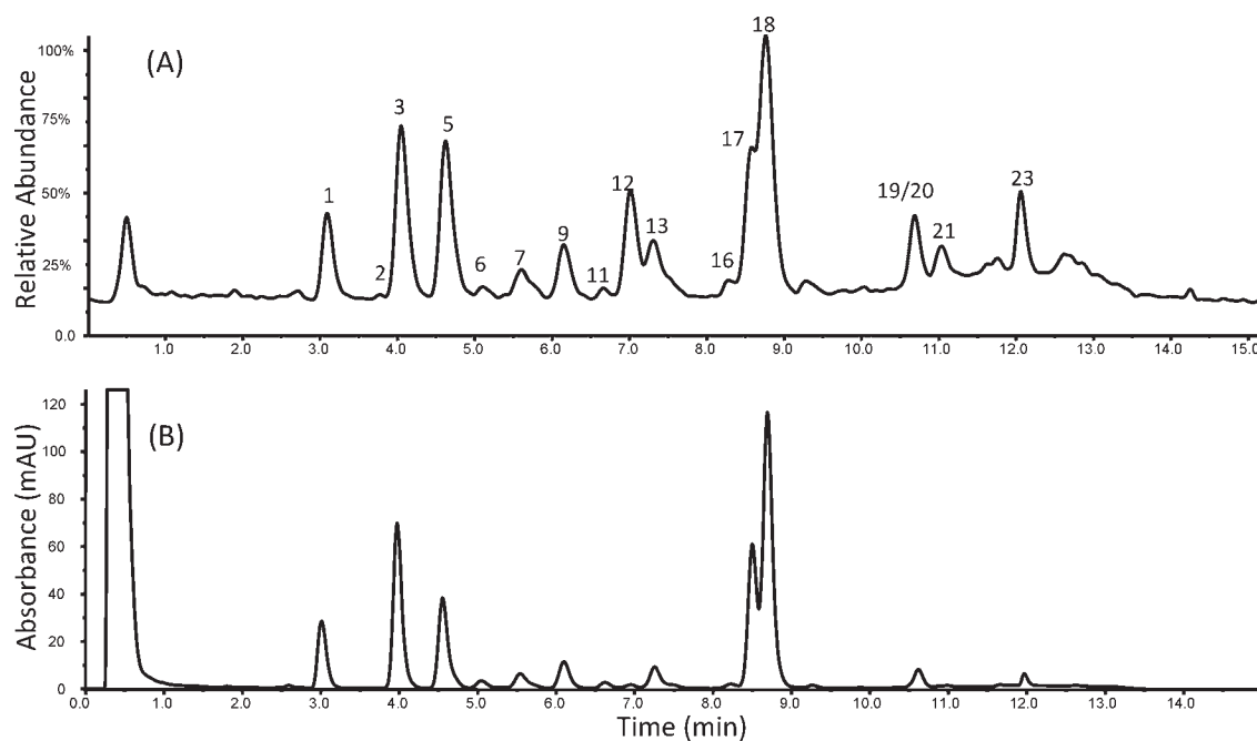
Figure 2. Separation of alkylamides from the root extract of Echinacea purpurea grown in Alberta by UFLC: TIC (A) and UV (B) at 254 nm. For peak assignment see Table 1.
