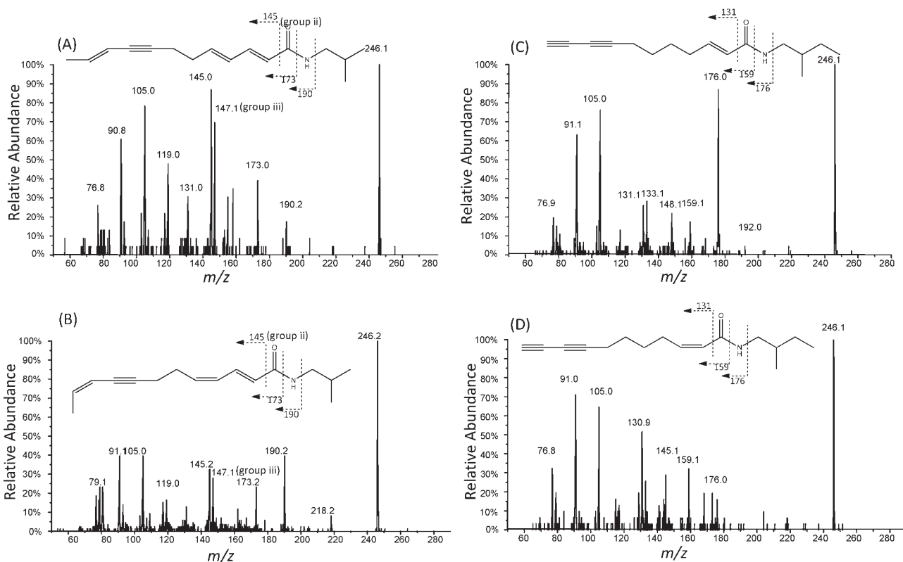
Figure 4. MS/MS spectra of isomeric alkylamide pairs with the molecular ion of m/z 246: (A) an isobutylamide eluting at 5.5 min; (B) an isobutylamide eluting at 5.7 min; (C) a 2-methylbutylamide eluting at 6.1 min; (D) a 2-methylbutylamide eluting at 7.2 min.
