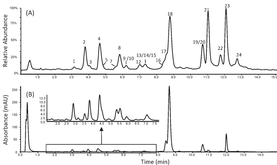
Figure 3. Separation of alkylamides from the root extract of Echinacea angustifolia from plants grown in Alberta by UFLC: TIC (A) and UV (B) at 254 nm. For peak assignment see Table 1.
