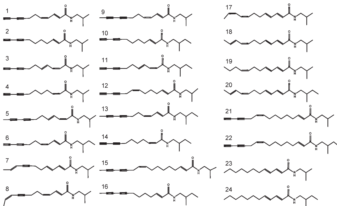
Figure 1. Structures of alkylamides found in Echinacea angustifolia and Echinacea purpurea roots. Compound numbering is based on the elution order using the UFLC method.
